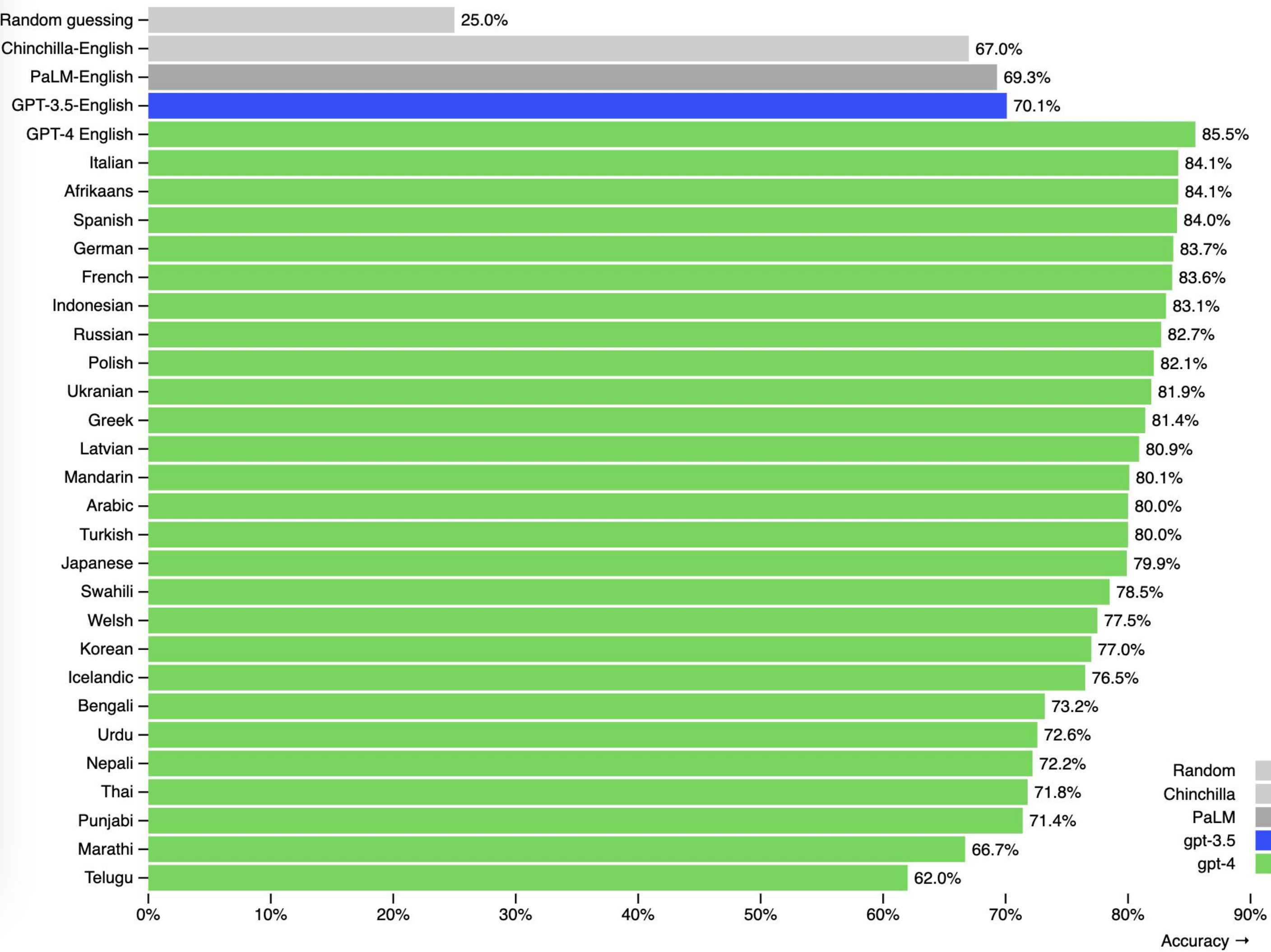
GPT-4 3-shot accuracy on MMLU across languages
